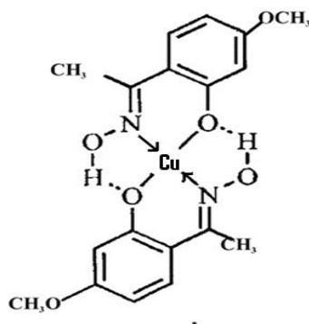
Proposed structure of Cu(II)-HMAOX complex
