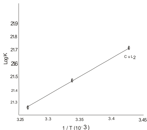
Fig 5. Kinetic linearization plot of the Cu(II)-HMAOX complex
