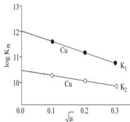
Fig 6. Extrapolation of \log K_n to zero ionic strength for Cu(II)-HMAOX interaction
