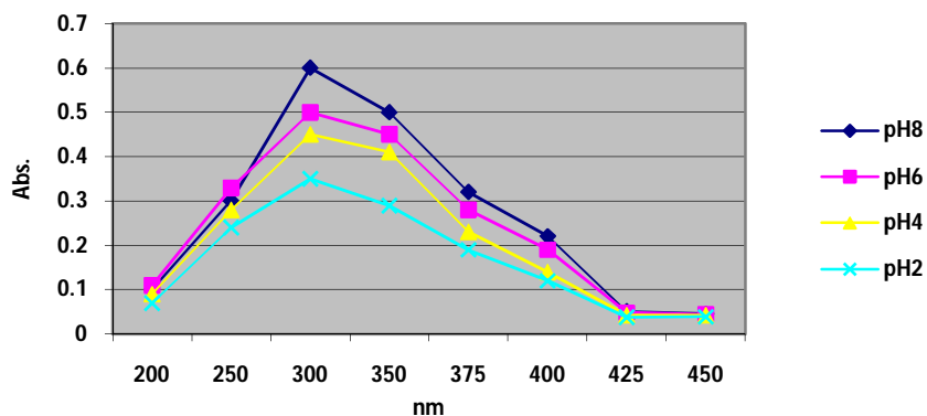
Fig. 2: UV-Vis. Spectra of Co(II) complex at different pH values.
