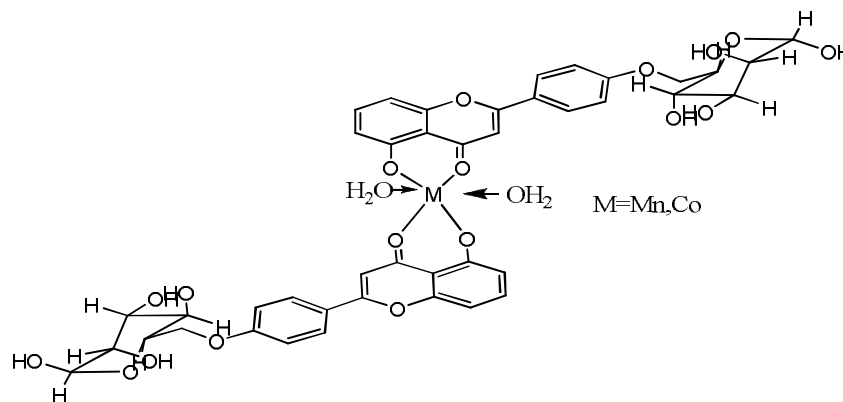
Fig. 1. Suggested structure of the Co(II) and Mn(II) complexes.
