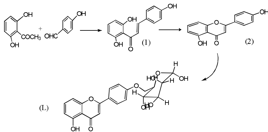
Scheme 1: Synthesis of Ligand
