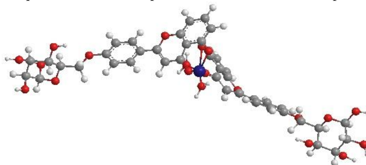
Fig 4. The optimized structural geometry of Co(II) complex
