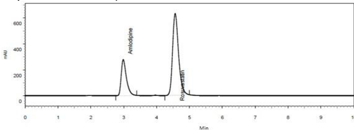
Fig.3 A typical HPLC Chromatogram showing the peak of Rosuvastatin calcium and Amlodipine besylate
