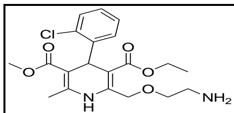
Fig.2 Chemical structure of Amlodipine besylate
