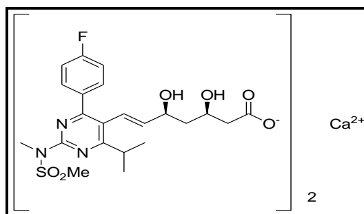
Fig.1 Chemical structure of Rosuvastatin calcium
