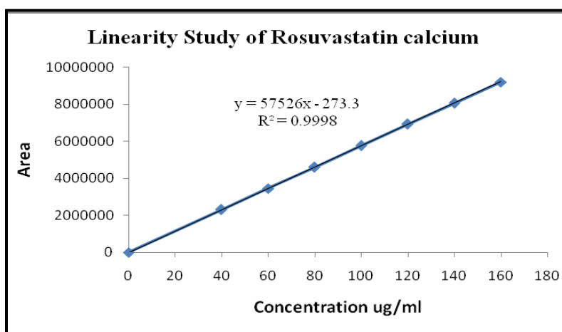
Fig 4. Calibration curve for Rosuvastatin calcium
