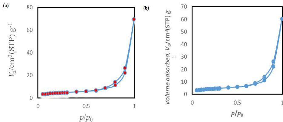
Figure 5. N2 adsorption-desorption isotherms for (a) SGP and (b) SGHP
