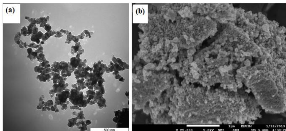
Figure 2. The (a) TEM and (b) FESEM images of ZnO prepared by sol-gel-hydrothermal method (SGHP)
