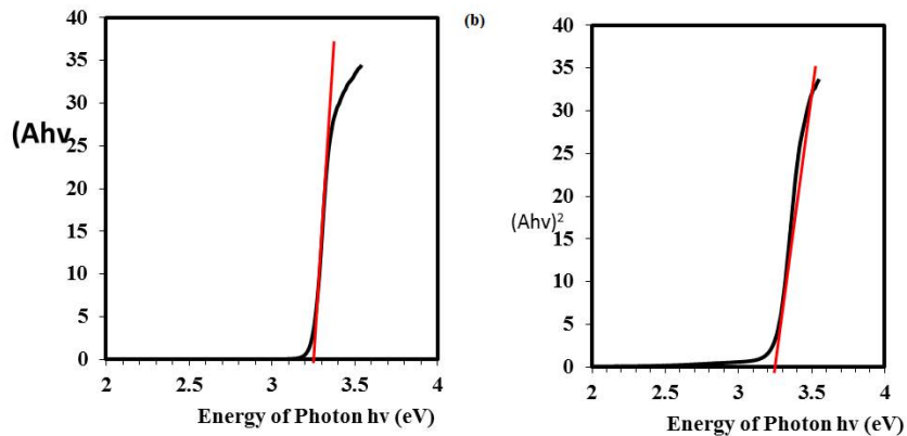
Figure 7. Band gap energy plot of (a) SGP1 and (b) SGHP
