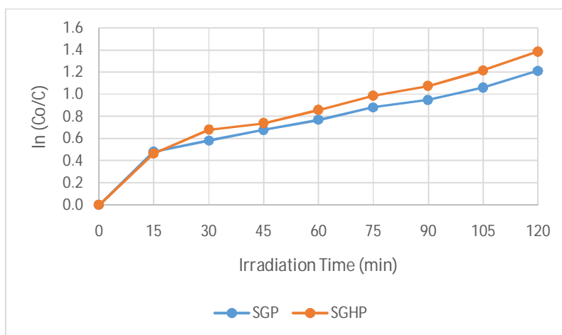
Figure 9. Kinetics of the degradation trend of NB by the ZnO samples synthesized using different methods
