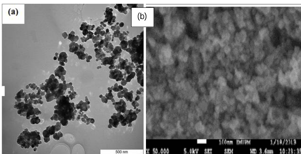
Figure 3. The (a) TEM and (b) FESEM images of ZnO prepared by sol-gel method (SGP)
