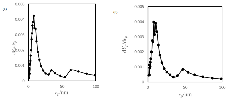
Figure 4. Pore size distribution of (a) SGP and (b) SGHP
